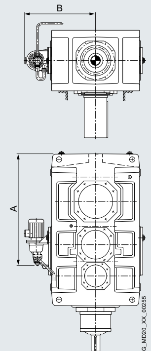
B3.V Forced lubrication by motor pump 2LP302-...12-....
