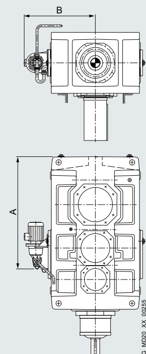
B3.V Forced lubrication by motor pump 2LP302-...12-....
