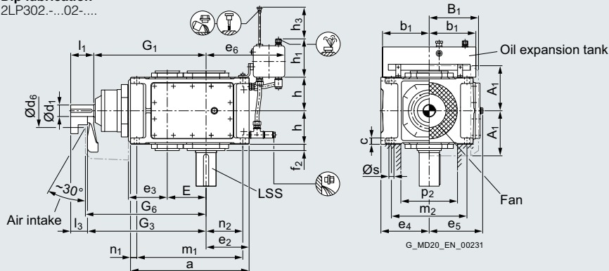
B2.V Forced lubrication by flange-mounted pump 2LP302-...02-....
