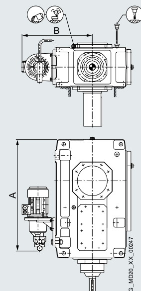
B3.V Forced lubrication by motor pump 2LP302-...12-....
