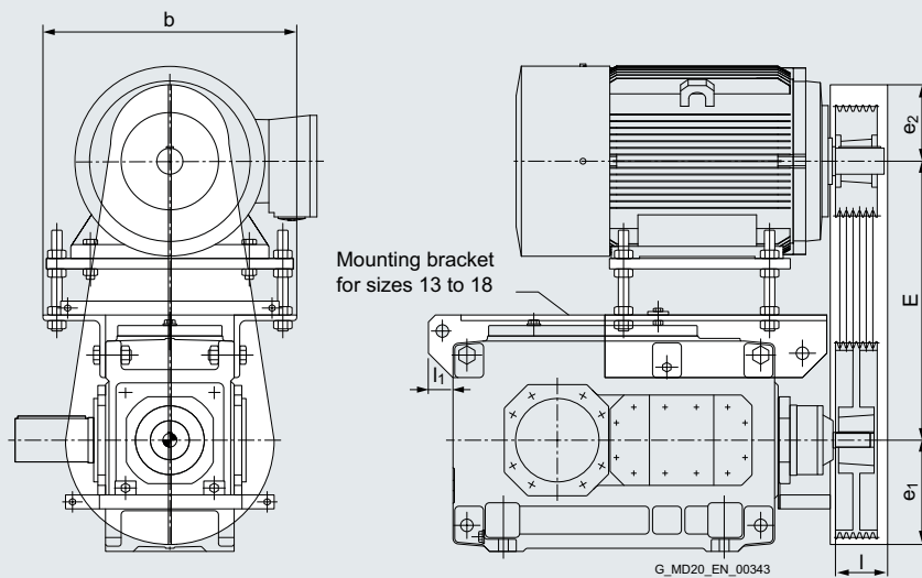
Piggy back for bevel helical gear unit, horizontal installation, types B3 and B4
