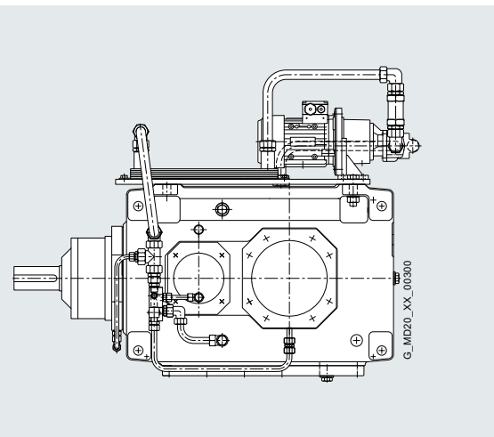
Example: B2SV08 with forced lubrication, motor pump and plate cooler (solution for variable speeds)
