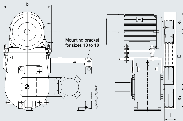
Piggy back for helical gear unit, horizontal installation, type H3
