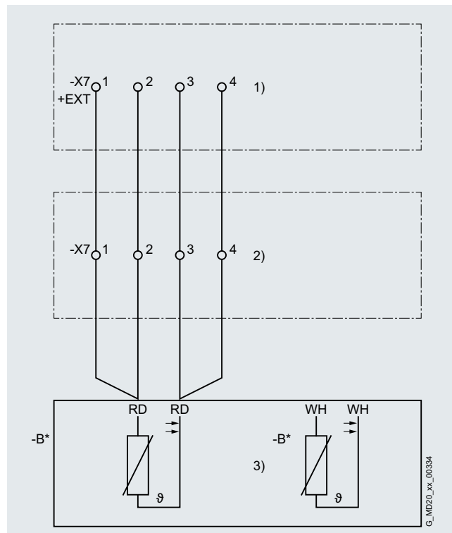
4-wire circuit
