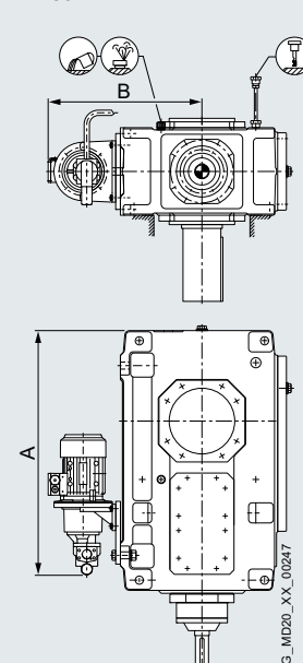
B3.V Forced lubrication by motor pump 2LP302-...12-....
