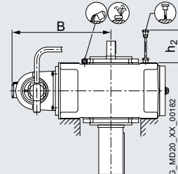
H3.V Forced lubrication by motor pump 2LP302-...52-....
