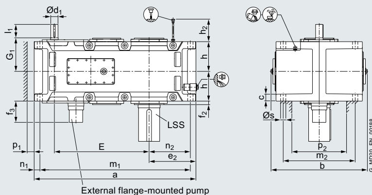
H3.V Forced lubrication by motor pump 2LP302-...52-....
