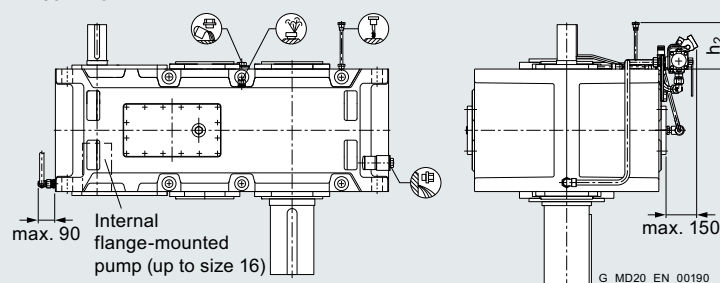
H3.V Forced lubrication by internal flange-mounted pump 2LP302-...52-....
