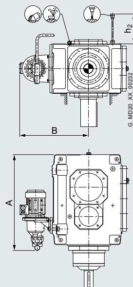
B2.V Forced lubrication by motor pump 2LP302-...02-....
