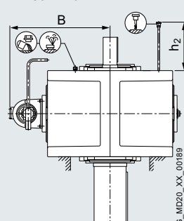
H3.V Forced lubrication by motor pump 2LP302-...52-....
