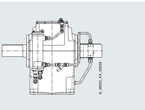
Example: H1SH09 with flange-mounted pump and oil-water cooler
