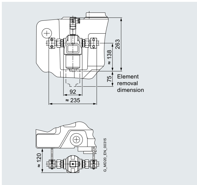
Line filter for types H2 and B2
