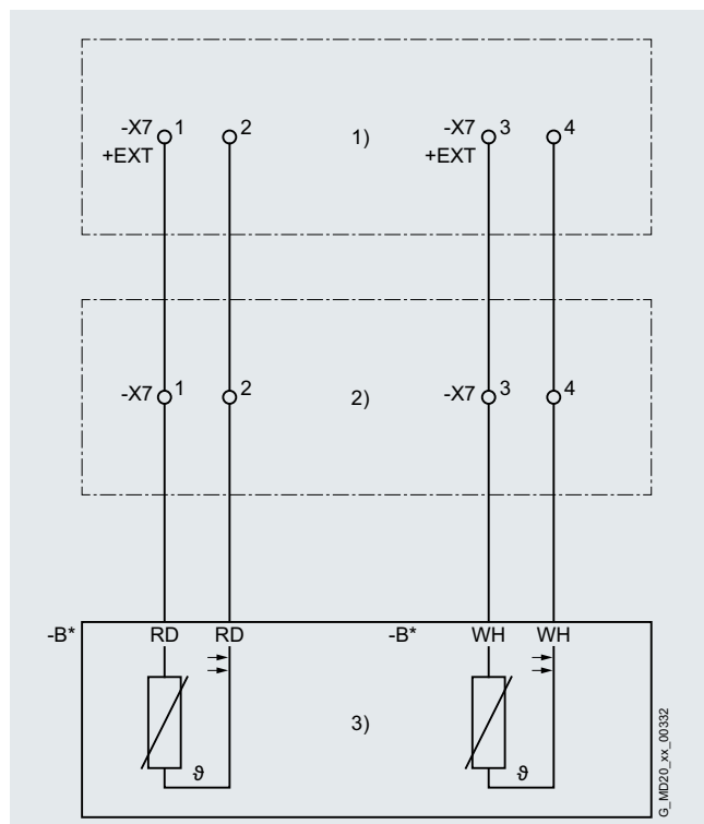
2-wire circuit
