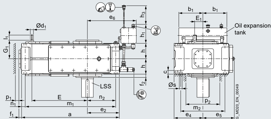
H4.V Forced lubrication by flange-mounted pump 2LP302-...62-....
