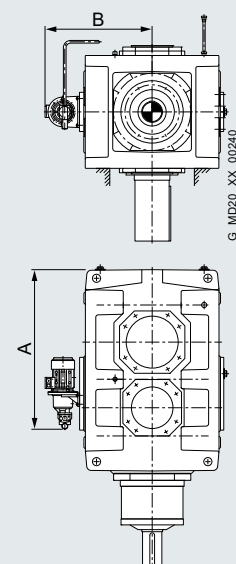
B2.V Forced lubrication by motor pump 2LP302-...02-....
