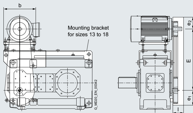
Piggy back for helical gear unit, horizontal installation, type H4
