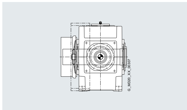
Example: B3DH15 with fan on brought out intermediate shaft
